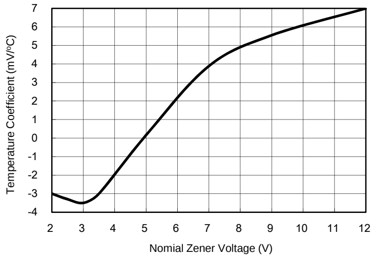
Fig. 1 Temperature Coefficients
