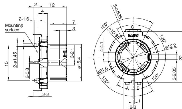
EC21C Reflow type Actuator length 12mm 15 pulse/30 detent
