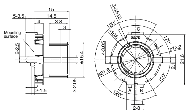
EC21A Actuator length 15mm 9 pulse/18 detent
