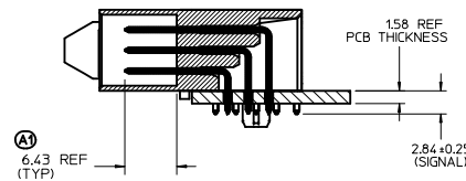
SECTION Z-Z
