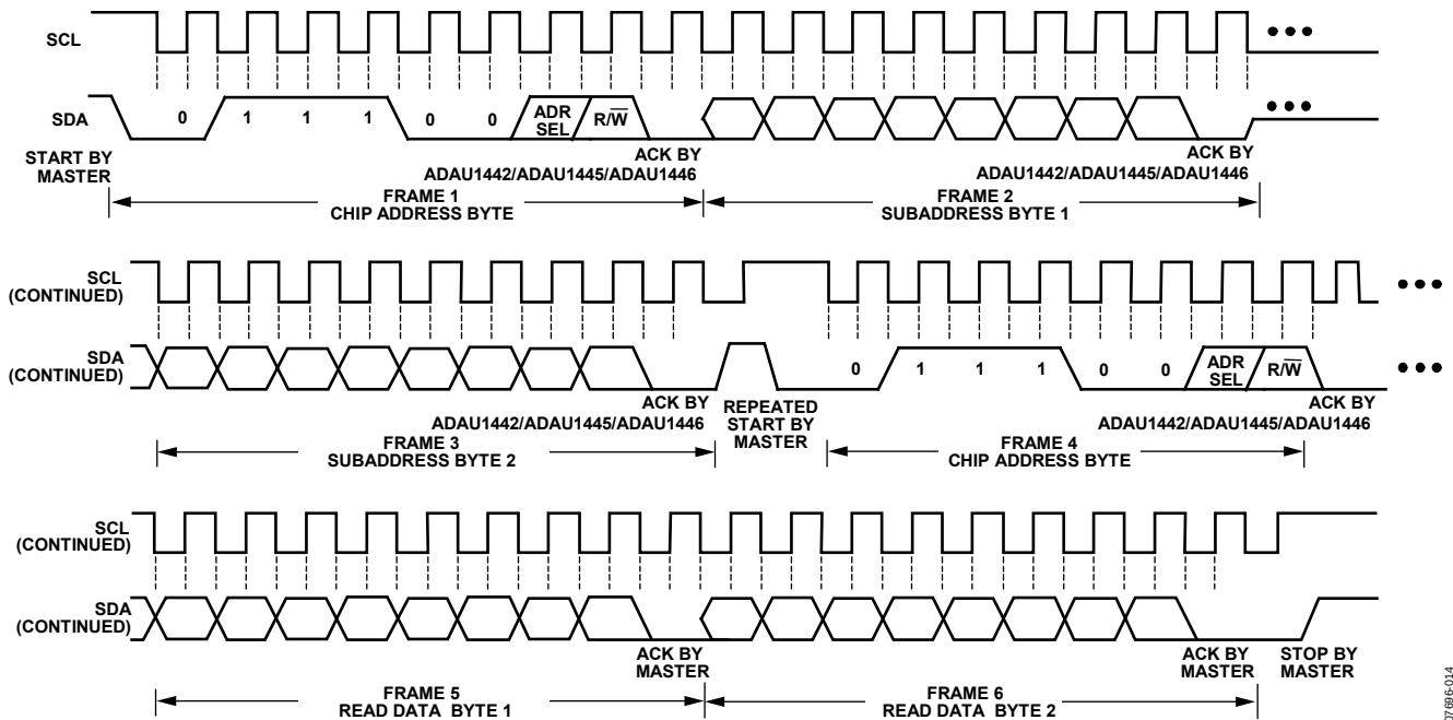
Figure 14. I²C Read Cloning
