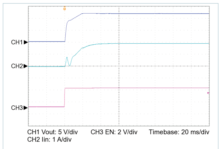
Figure 14 — Startup from EN, V_{IN} = 270\text{ V} , C_{OUT\_EXT} = 10000\text{ }\mu\text{F} , R_{LOAD} = 0.288\text{ }\Omega
