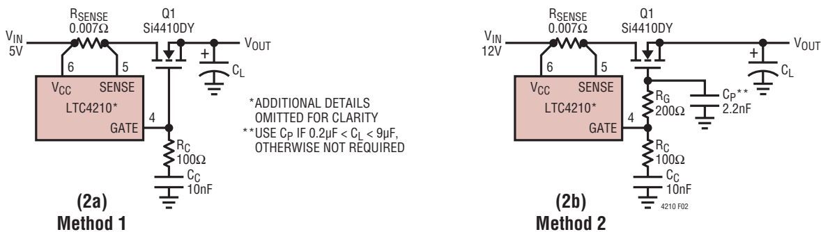
Figure 2. Frequency Compensation
