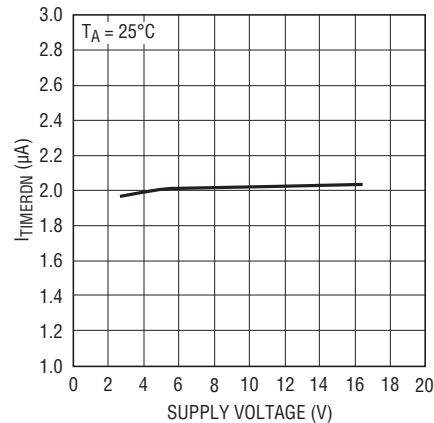
I_{TIMERDN} (In Cool-Off Cycle) vs Supply Voltage
