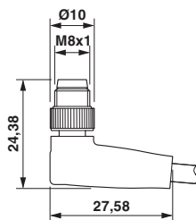
Dimensional drawing
