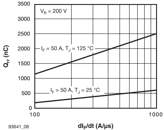
93641_08 di_F/dt (A/μs) Fig. 8 - Typical Stored Charge vs. di_F/dt
