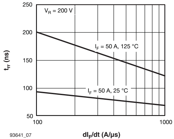
93641_07 di_F/dt (A/μs) Fig. 7 - Typical Reverse Recovery Time vs. di_F/dt
