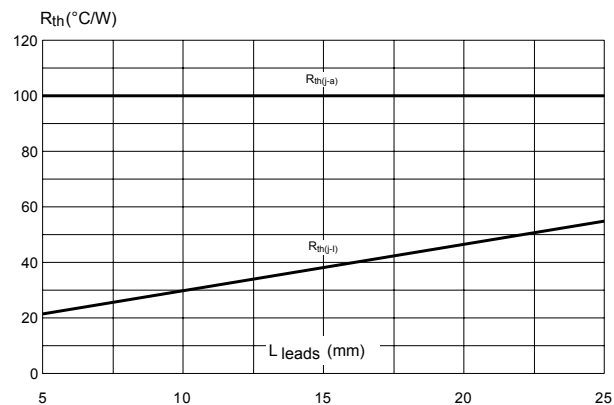
Figure 12. Thermal resistance versus lead length (DO-15)
