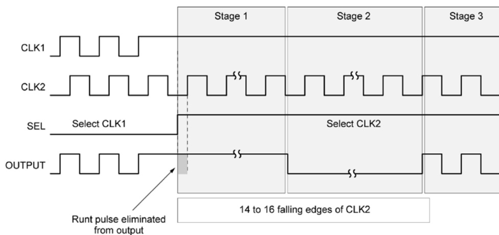
Timing Diagram 2
