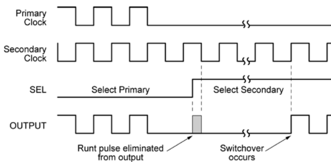
Simplified Example Illustrating Runt Pulse Eliminator (RPE) when Primary Clock Fails
