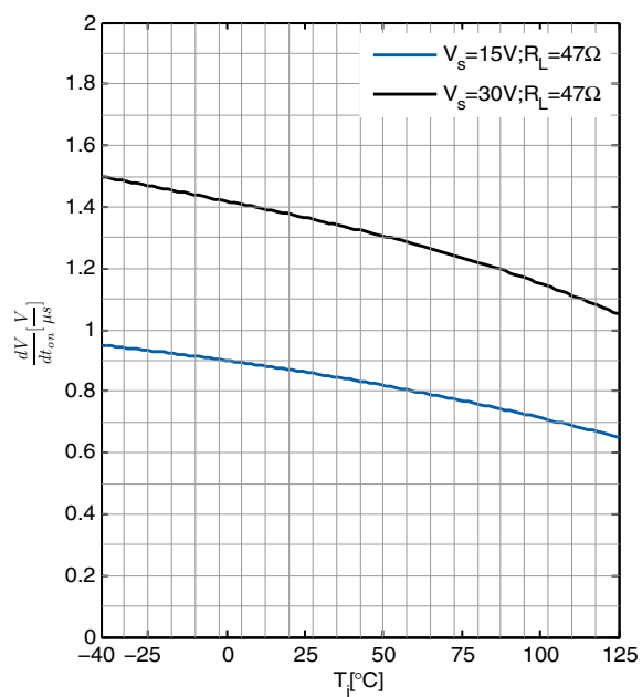
ON Slewrate SR_{ON} versus Junction Temperature T_j
