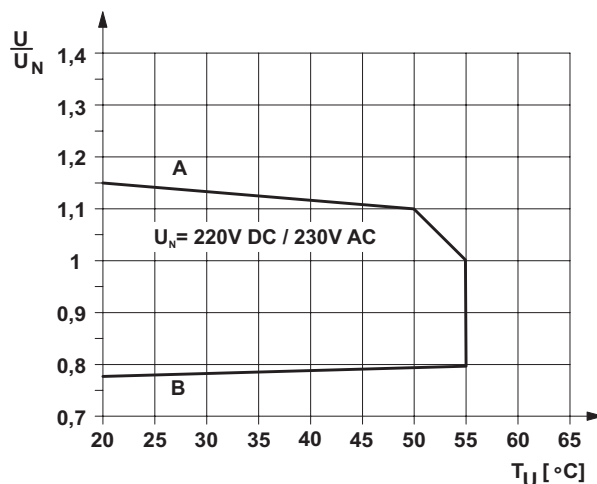
Figure 3 Operating voltage range for 230 V AC/DC
