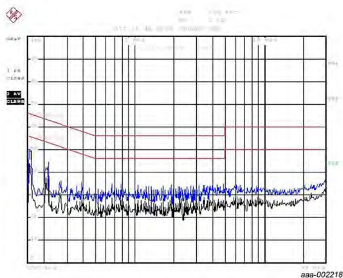
a. EMI at 115 V (AC) input voltage and 2 W output at 80 % load.
