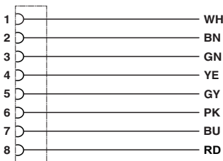
Contact assignment of M8 socket
