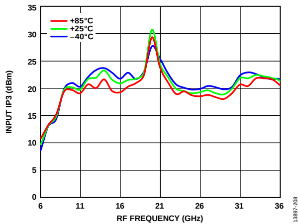
Figure 8. Input IP3 vs. RF Frequency over Various Temperatures, P_{LO} = 15 dBm
