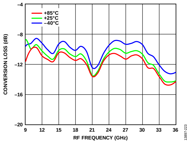
Figure 23. Conversion Loss vs. RF Frequency over Various Temperatures, P_{LO} = 15 dBm
