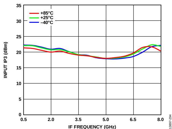
Figure 82. Input IP3 vs. IF Frequency over Various Temperatures, P_{LO} = 15 dBm
