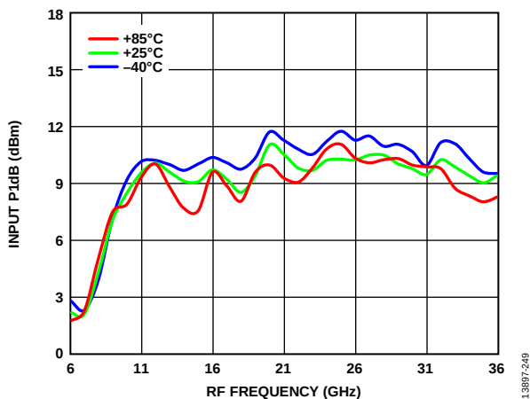
Figure 49. Input P1dB vs. RF Frequency over Various Temperatures, P_{LO} = 15 dBm
