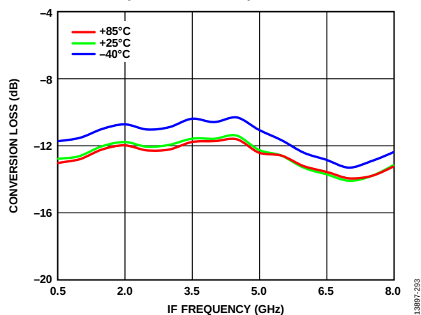
Figure 81. Conversion Loss vs. IF Frequency over Various Temperatures, P_{LO} = 15 dBm
