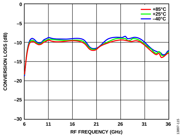
Figure 47. Conversion Loss vs. RF Frequency over Various Temperatures, P_{LO} = 15 dBm
