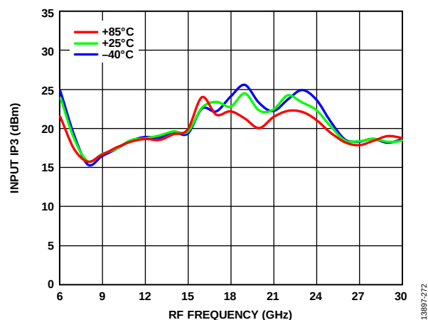
Figure 72. Input IP3 vs. RF Frequency over Various Temperatures, P_{LO} = 15 dBm
