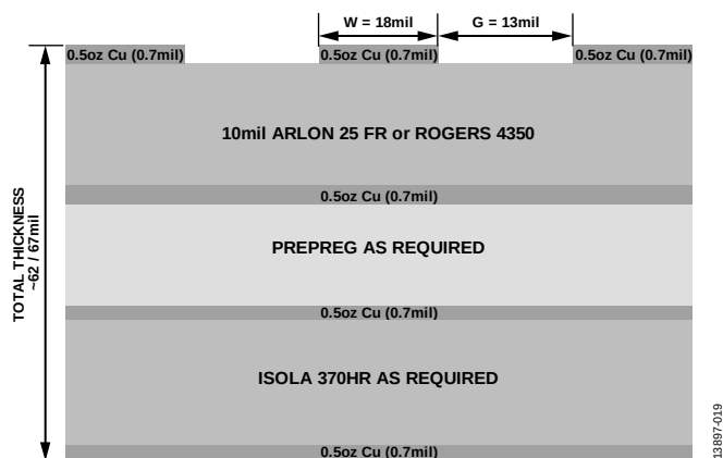
Figure 94. Evaluation Board Cross Sectional View
