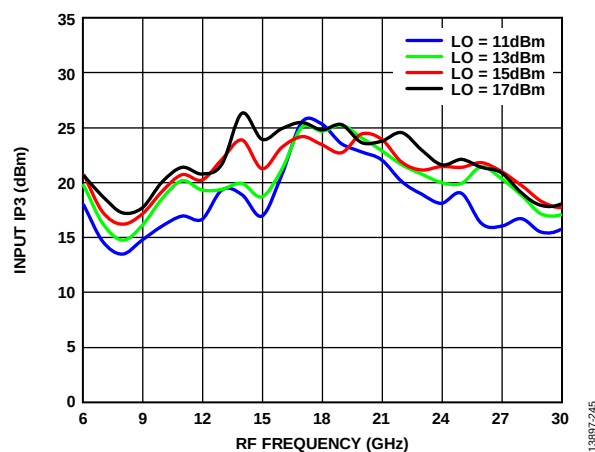
Figure 45. Input IP3 vs. RF Frequency over Various LO Drives
