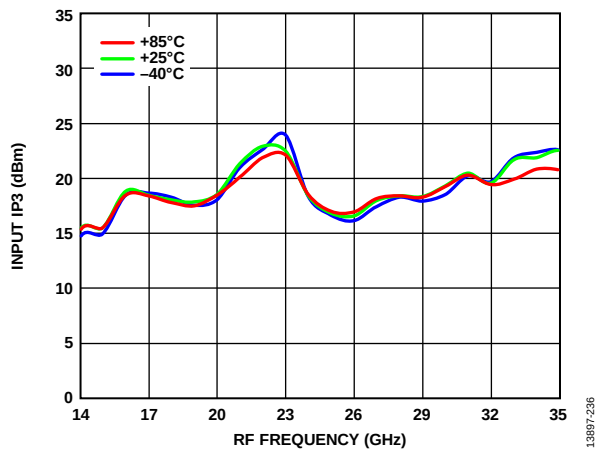
Figure 36. Input IP3 vs. RF Frequency over Various Temperatures, P_{LO} = 15 dBm
