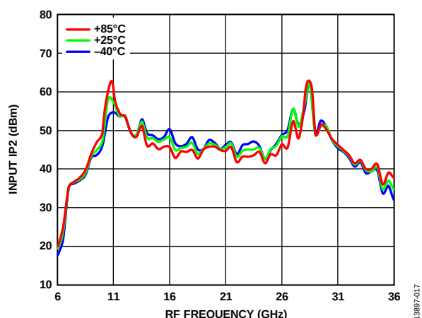
Figure 17. Input IP2 vs. RF Frequency over Various Temperatures, P_{LO} = 15 dBm
