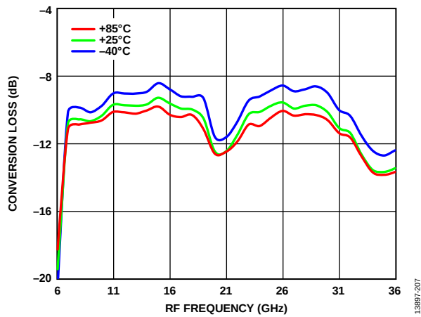
Figure 7. Conversion Loss vs. RF Frequency over Various Temperatures, P_{LO} = 15 dBm
