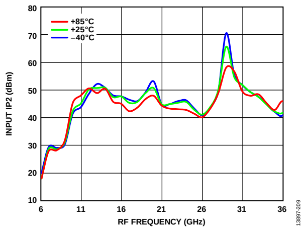
Figure 9. Input IP2 vs. RF Frequency over Various Temperatures, P_{LO} = 15 dBm
