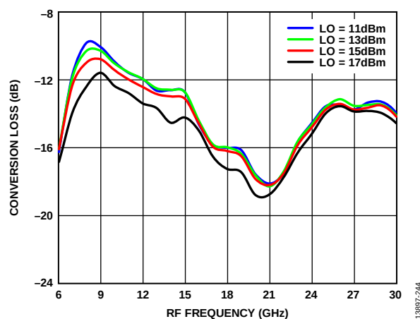
Figure 44. Conversion Loss vs. RF Frequency over Various LO Drives
