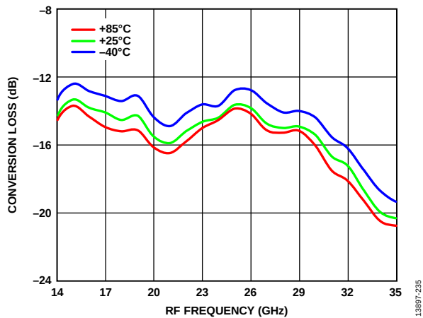
Figure 35. Conversion Loss vs. RF Frequency over Various Temperatures, P_{LO} = 15 dBm
