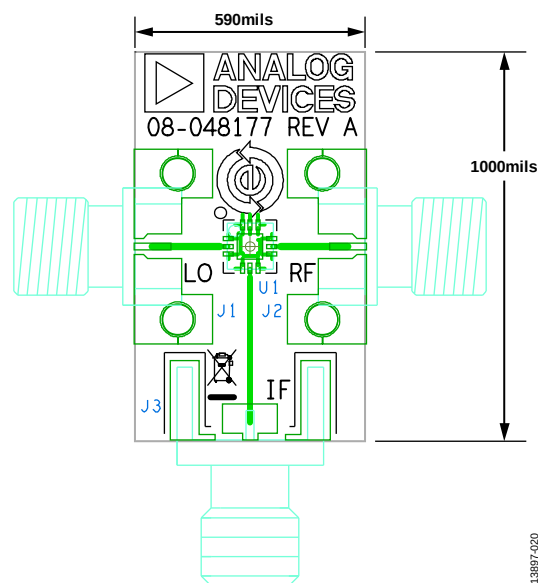
Figure 95. EV1HMC774ALC3B Evaluation Board
