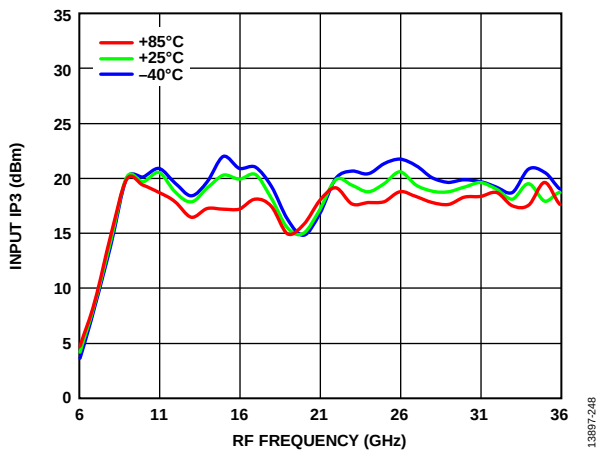
Figure 48. Input IP3 vs. RF Frequency over Various Temperatures, P_{LO} = 15 dBm
