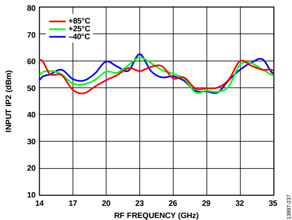
Figure 37. Input IP2 vs. RF Frequency over Various Temperatures, P_{LO} = 15 dBm
