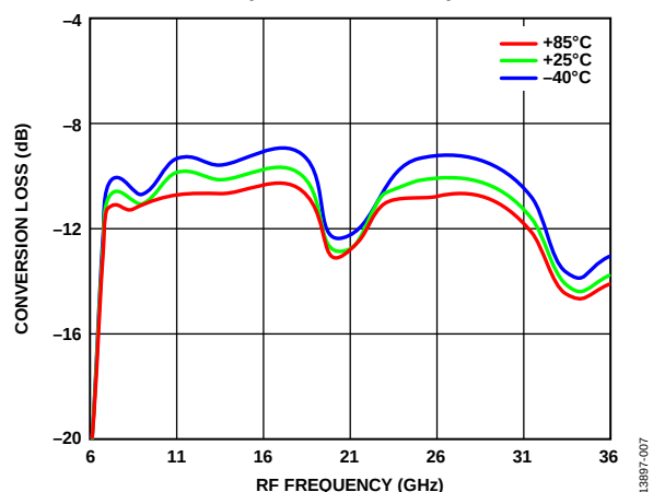
Figure 15. Conversion Loss vs. RF Frequency over Various Temperatures, P_{LO} = 15 dBm
