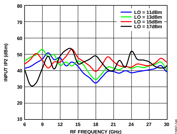
Figure 46. Input IP2 vs. RF Frequency over Various LO Drives
