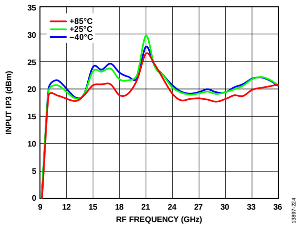
Figure 24. Input IP3 vs. RF Frequency over Various Temperatures, P_{LO} = 15 dBm
