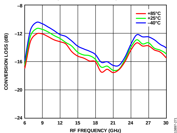
Figure 71. Conversion Loss vs. RF Frequency over Various Temperatures, P_{LO} = 15 dBm
