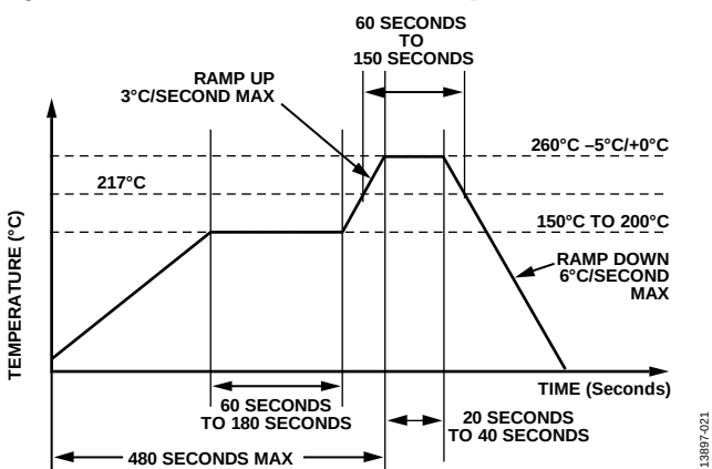
Figure 96. Pb-Free Reflow Solder Profile
