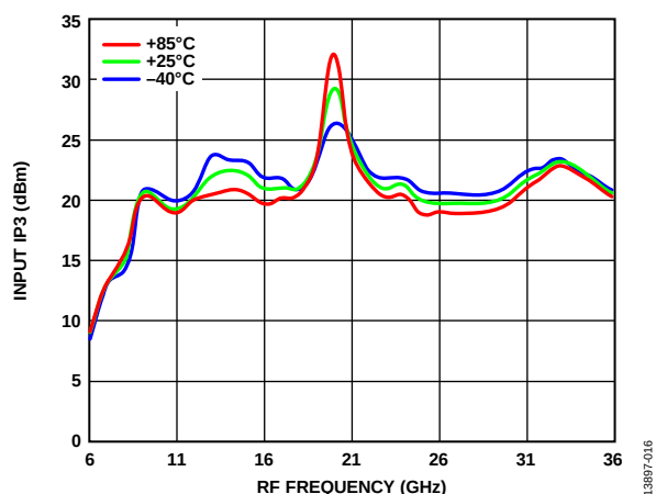
Figure 16. Input IP3 vs. RF Frequency over Various Temperatures, P_{LO} = 15 dBm
