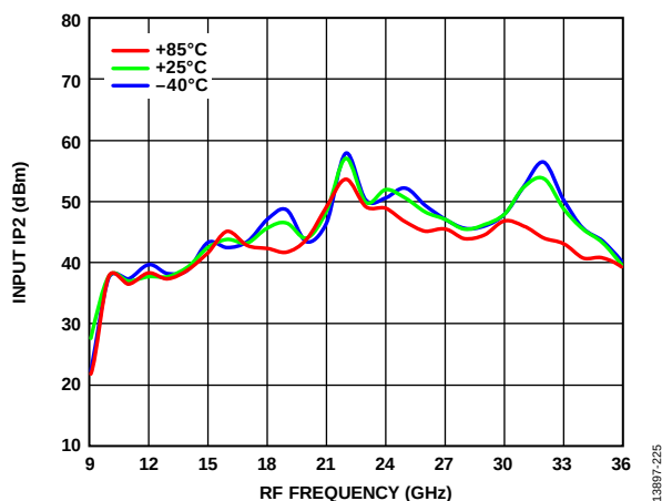
Figure 25. Input IP2 vs. RF Frequency over Various Temperatures, P_{LO} = 15 dBm
