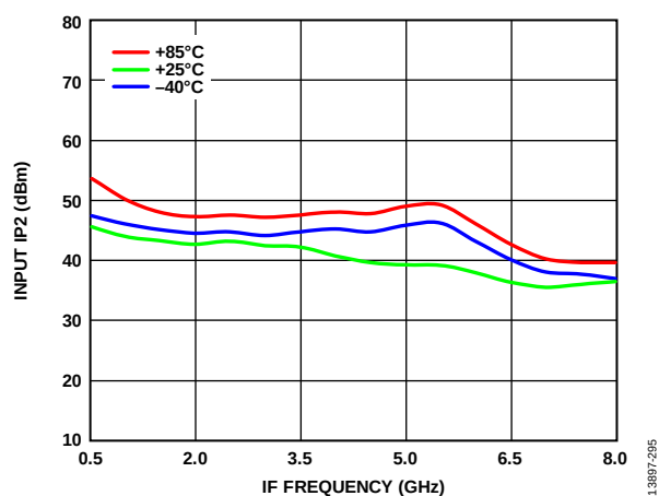
Figure 83. Input IP2 vs. IF Frequency over Various Temperatures, P_{LO} = 15 dBm
