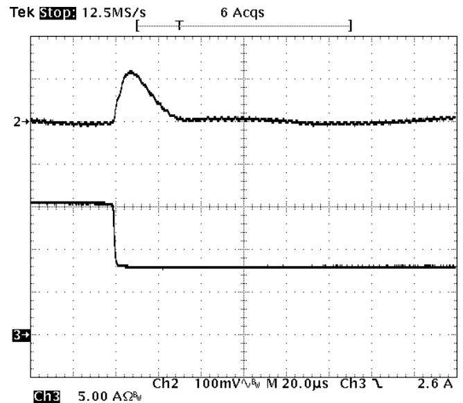
Fig-1.0V-7: Output voltage response for Vout=1.0V to negative load current step change from 16A to 8A with slew rate of -5A/us at Vin=12V. Co=47uFx4 ceramic. Top trace: output voltage (100mV/div.) Bottom trace: load current (5A/div.) Time scale: 20us/div.
