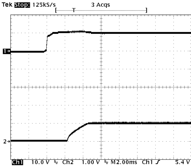
Fig-1.0V-4: Turn-on transient for Vout=1.0V with application of Vin at full rated load current (resistive) and 47uFx4 external capacitance at Vin=12V. Top trace: Vin (10V/div.) Bottom trace: output voltage (1V/div.) Time scale: 2 ms/div.
