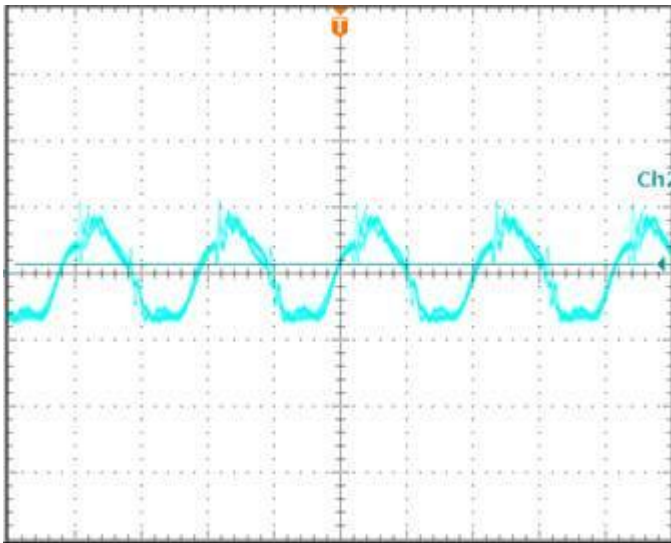
Figure 12: Input reflected ripple current, i_s , through a 12\mu\text{H} source inductor at nominal input voltage and max load current ( 25\text{mA/div} \times 4\mu\text{s/div} ).
