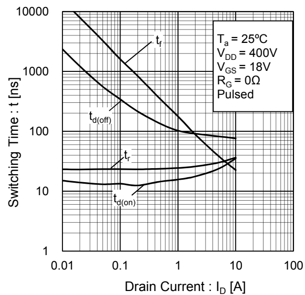
Fig.17 Switching Characteristics
