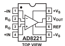
Figure 44. Pinout Diagram
