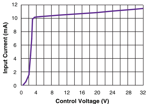
Figure 3c — SH60D relays
