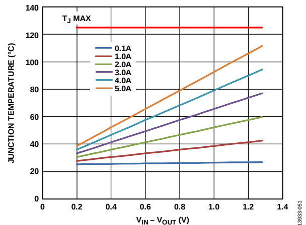
Figure 51. 500 mm 2 of PCB Copper, T_B = 25^\circ\text{C}
