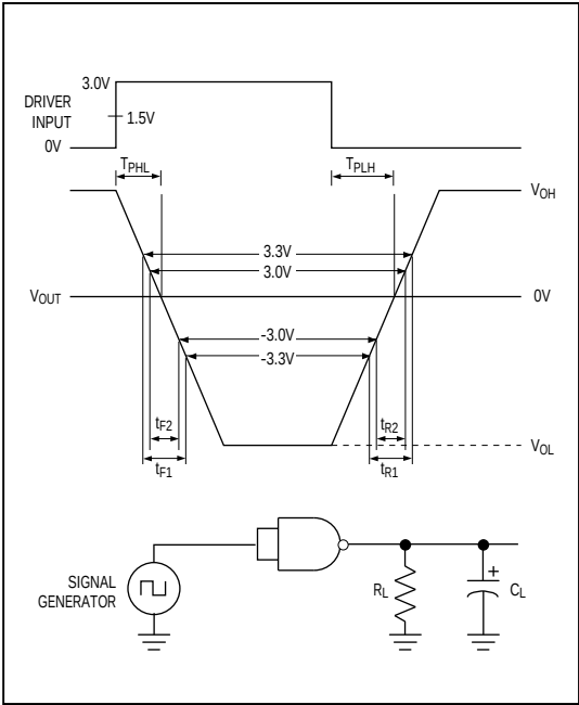
Figure 3. Slew-Rate Test Circuit and Timing Diagram
