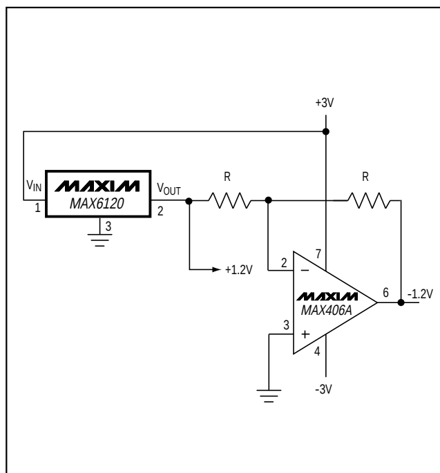
Figure 2. Low-Power \pm 1.2V Reference
