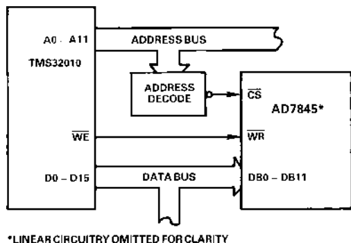
Figure 21. TMS32010
