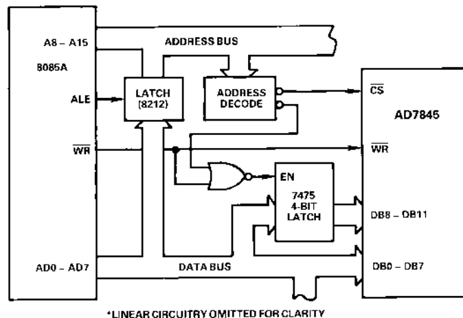
Figure 22. 8085A Interface
