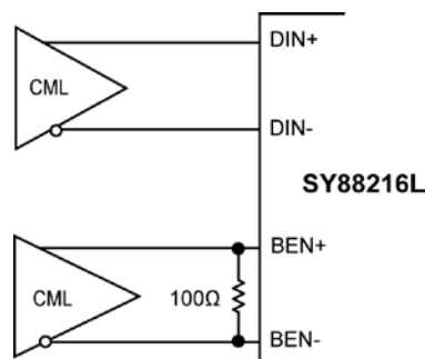
Figure 2b. Driving DIN and BEN with CML Outputs
