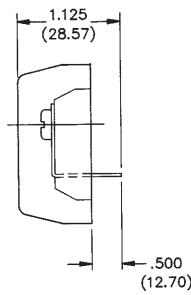
“Y” Terminals
