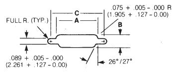
Figure 2. Rear Mounting
