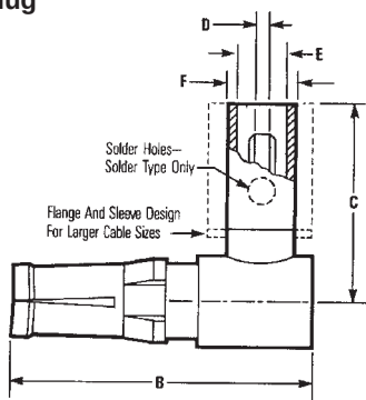
Plug
