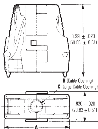
Adapter Hood with Latches
