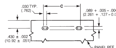
Figure 3. Edgeboard Mounting
