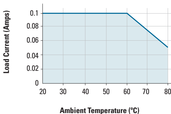
DERATE CURVES:
