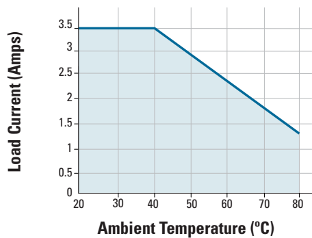
DERATE CURVES:
