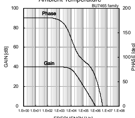
Fig.92 Gain – Frequency
