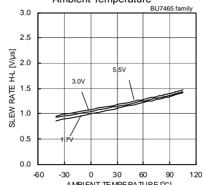
Fig.91 Slew Rate H-L – Ambient Temperature
