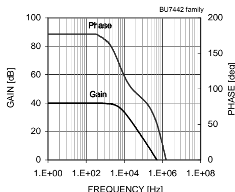
Fig.138 Gain – Frequency
