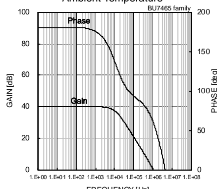
Fig.92 Gain – Frequency
