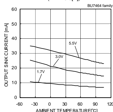
Fig.58 Output Sink Current – Ambient Temperature ( V_{OUT}=V_{SS}+0.4[V] )
