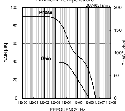
Fig.92 Gain – Frequency
