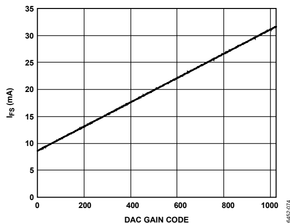
Figure 77. I_{\text{FS}} vs. DAC Gain Code
