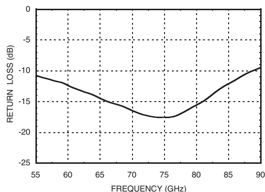
“On” Output Return Loss vs. Freq. CTLA= -5V, CTLB= 5V for RFOUT1 to be ON
