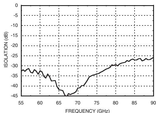
“Off” Isolation vs. Freq. CTLA= +5V, CTLB= -5V for RFOUT1 to be OFF
