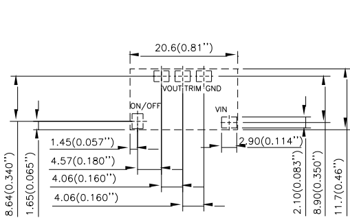
RECOMMAND PWB PAD LAYOUT
