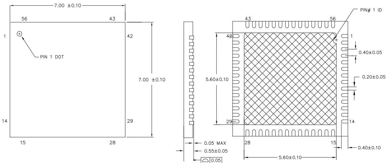
BOTTOM VIEW
