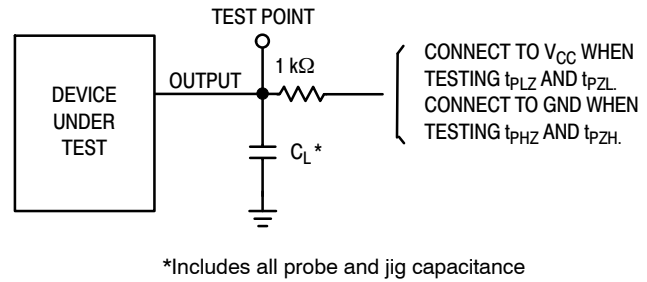
Figure 7. Test Circuit
