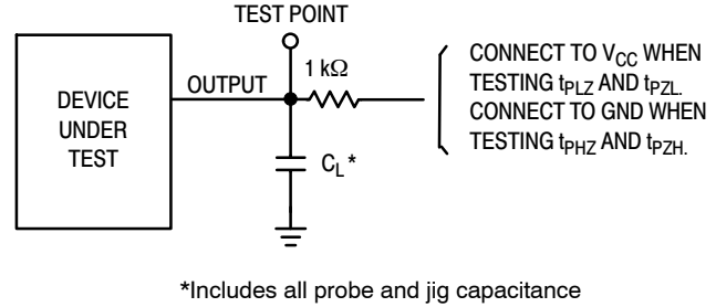
Figure 7. Test Circuit
