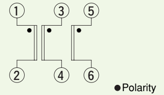
Figure 35. Circuit diagram
