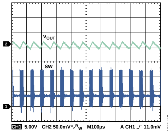
Figure 29. Steady State Waveform at Light Load, V_{IN} = 12\text{ V} , V_{OUT} = 3.3\text{ V} , I_{OUT} = 30\text{ mA} , f_{SW} = 600\text{ kHz} , L = 4.7\text{ μH} , C_{OUT} = 47\text{ μF} \times 2 , Automatic PWM/PSM Mode
