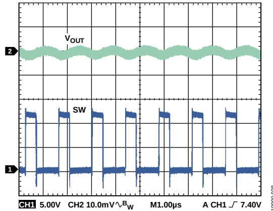
Figure 28. Steady State Waveform at Heavy Load, V_{IN} = 12\text{ V} , V_{OUT} = 3.3\text{ V} , I_{OUT} = 3\text{ A} , f_{SW} = 600\text{ kHz} , L = 4.7\text{ μH} , C_{OUT} = 47\text{ μF} \times 2 , FPWM Mode
