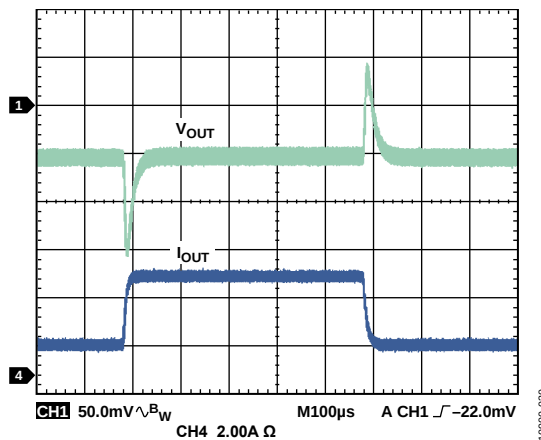
Figure 30. Channel 1/Channel 2 Load Transient, 1 A to 4 A, V_{IN} = 12\text{ V} , V_{OUT} = 3.3\text{ V} , f_{SW} = 600\text{ kHz} , L = 2.2\text{ μH} , C_{OUT} = 47\text{ μF} \times 2
