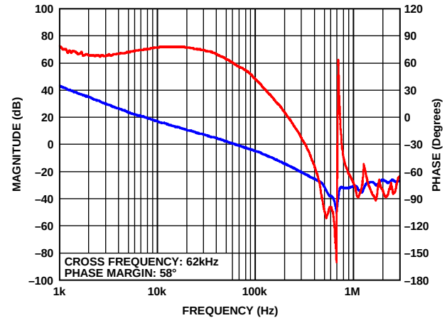
Figure 50. Bode Plot for 1.2 V Output
