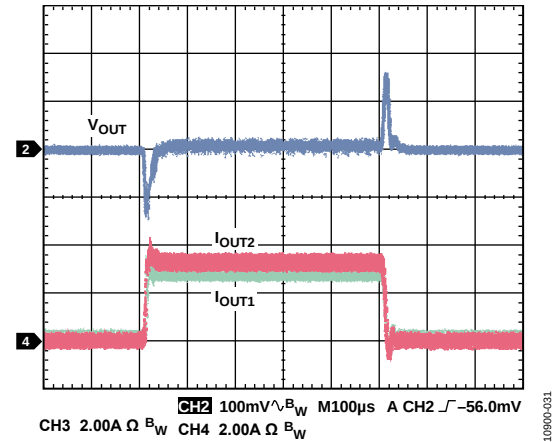
Figure 31. Load Transient, Channel 1/Channel 2 Parallel Output, 0 A to 6 A, V_{IN} = 12\text{ V} , V_{OUT} = 3.3\text{ V} , f_{SW} = 600\text{ kHz} , L = 4.7\text{ μH} , C_{OUT} = 47\text{ μF} \times 4
