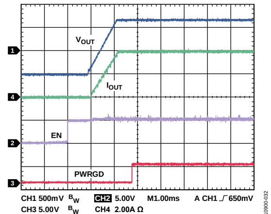
Figure 32. Channel 1/Channel 2 Soft Start with 4 A Resistance Load, V_{IN} = 12\text{ V} , V_{OUT} = 1.2\text{ V} , f_{SW} = 600\text{ kHz} , L = 1\text{ μH} , C_{OUT} = 47\text{ μF} \times 2
