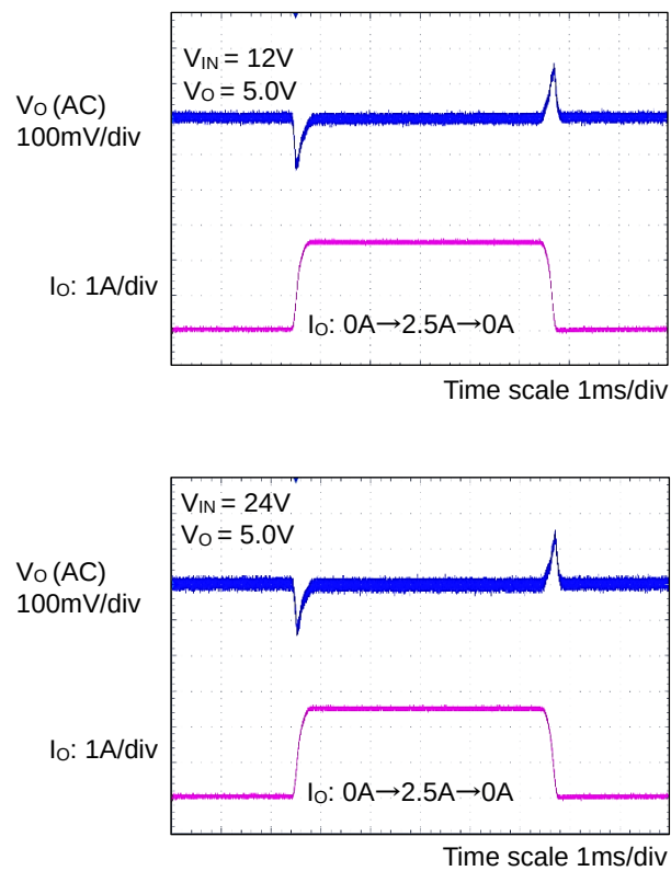
Figure 12. Load Transient Characteristics
