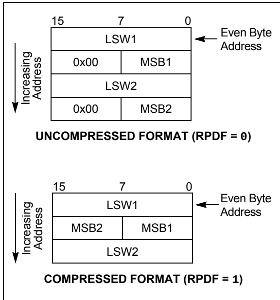
FIGURE 3-15: UNCOMPRESSED/COMPRESSED FORMAT
