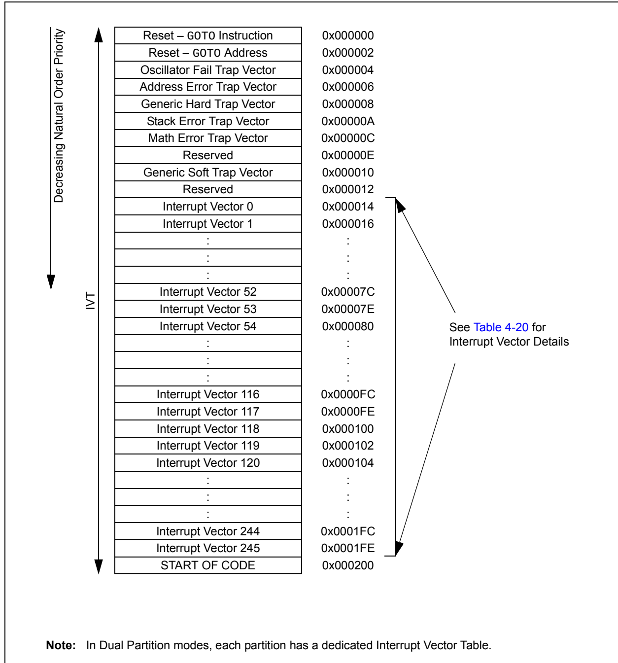
FIGURE 4-16: dsPIC33CH128MP508S1 FAMILY INTERRUPT VECTOR TABLE
