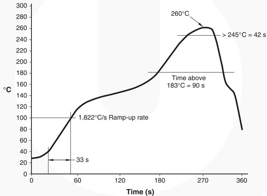
Figure 13. Reflow Profile
