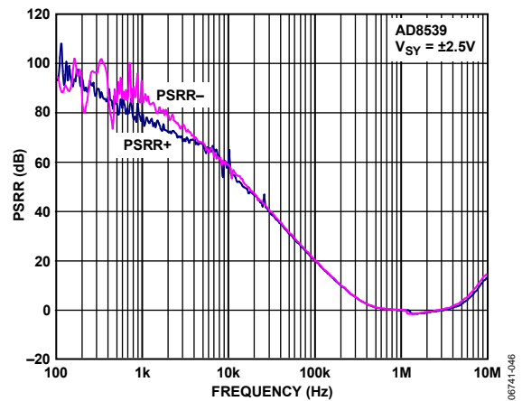
Figure 45. AD8539 PSRR vs. Frequency
