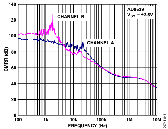
Figure 44. AD8539 CMRR vs. Frequency
