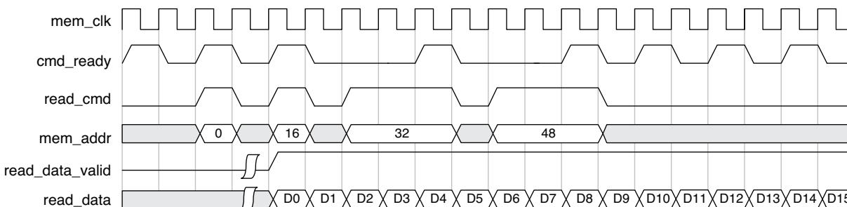
Figure 2-13. Timing Diagram for Memory Read
