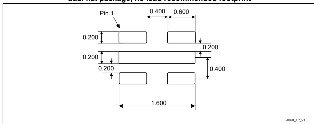
Figure 19. UDFPN5 - 5-lead, 1.7 × 1.4 mm, 0.55 mm thickness, ultra thin fine pitch dual flat package, no lead recommended footprint
